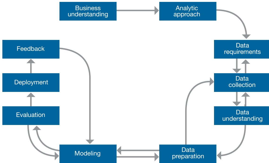
Figure 1. Foundational Methodology for Data Science.
